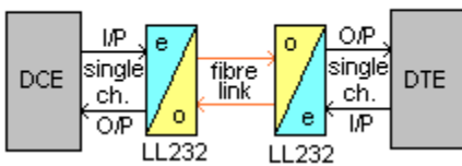
Single channel RS232 fibre interface
